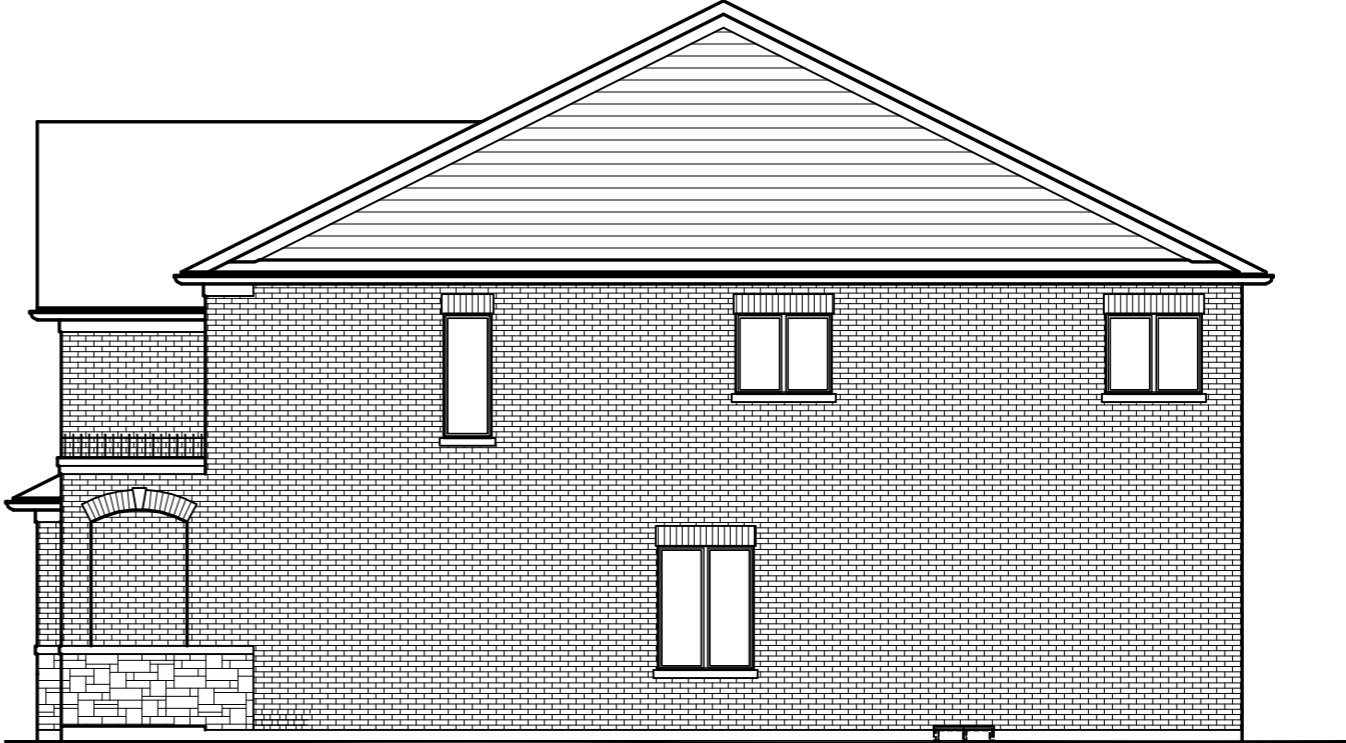
RIGHT SIDE ELEVATION 'B'
