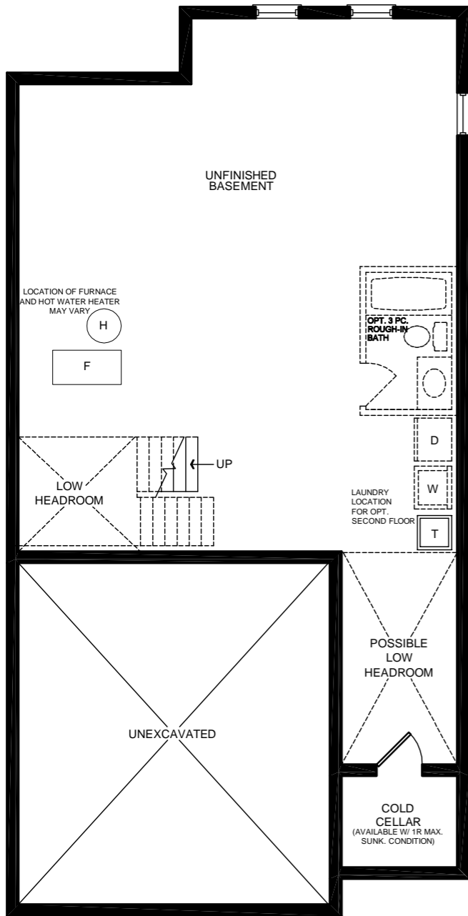
BASEMENT FLOOR ELEV. 'A'
