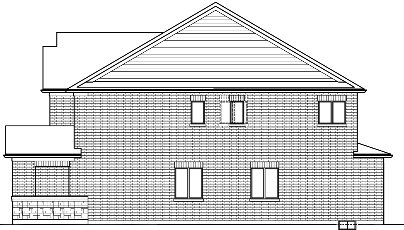
RIGHT SIDE ELEVATION 'B'
