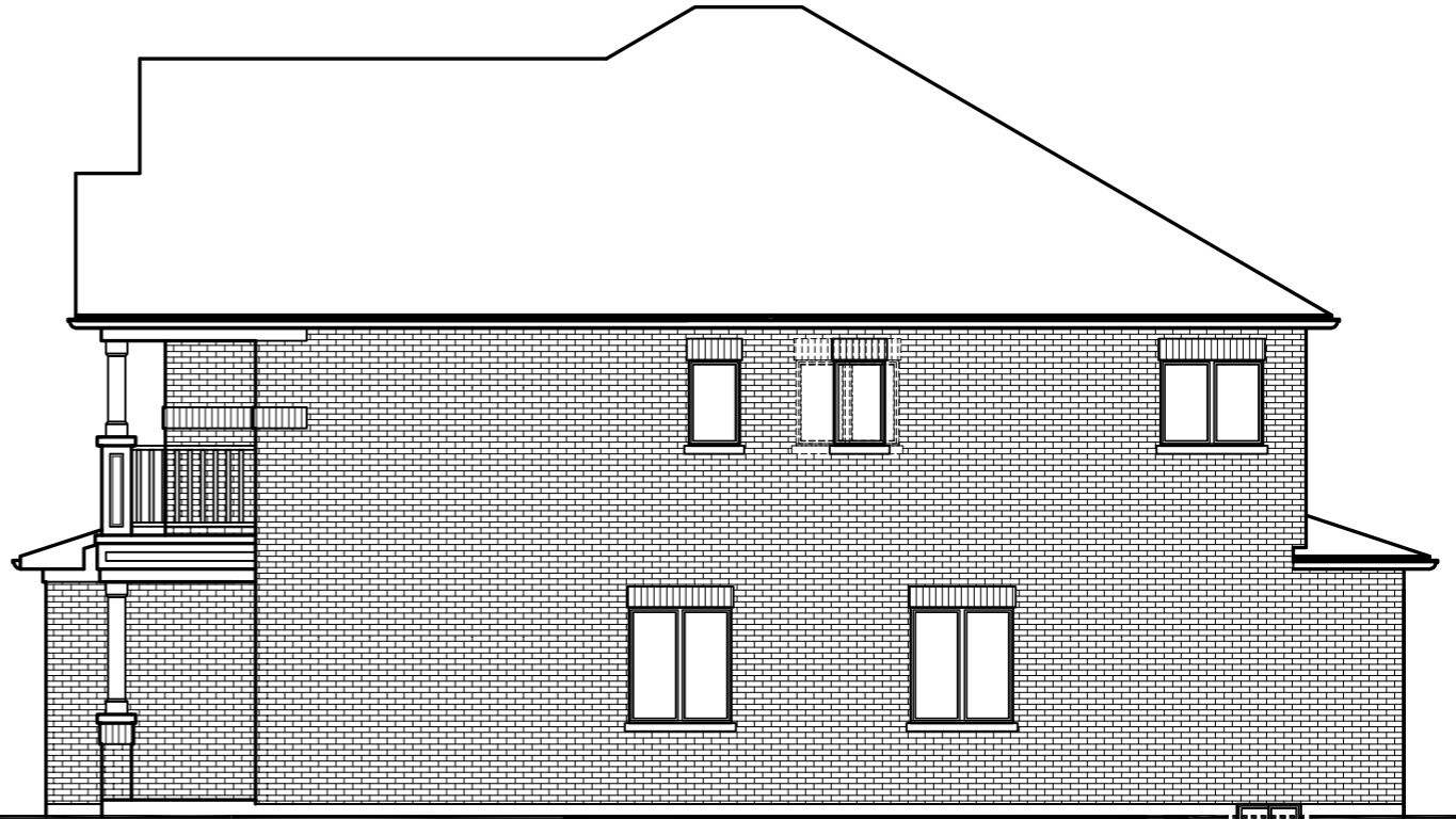
RIGHT SIDE ELEVATION 'A'
