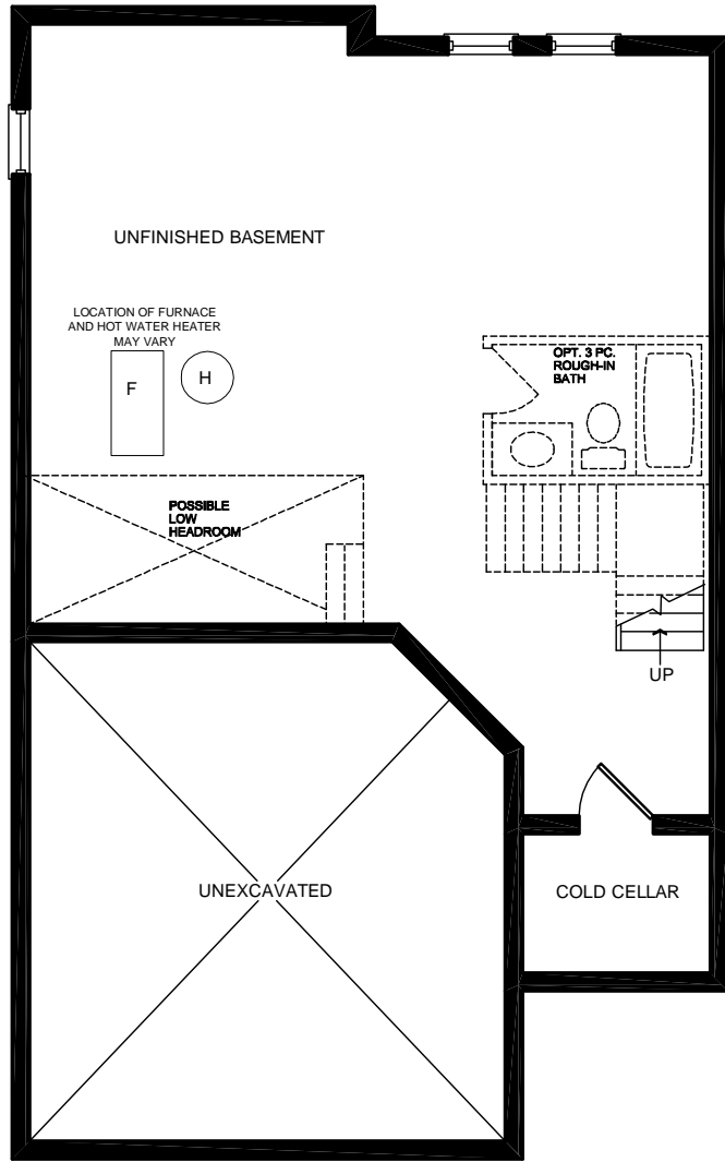
BASEMENT FLOOR ELEV. 'A & B'
