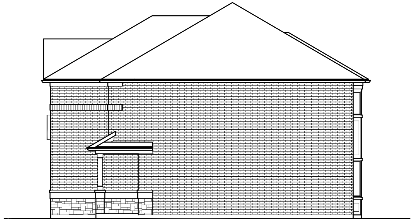
RIGHT SIDE ELEVATION 'B'
